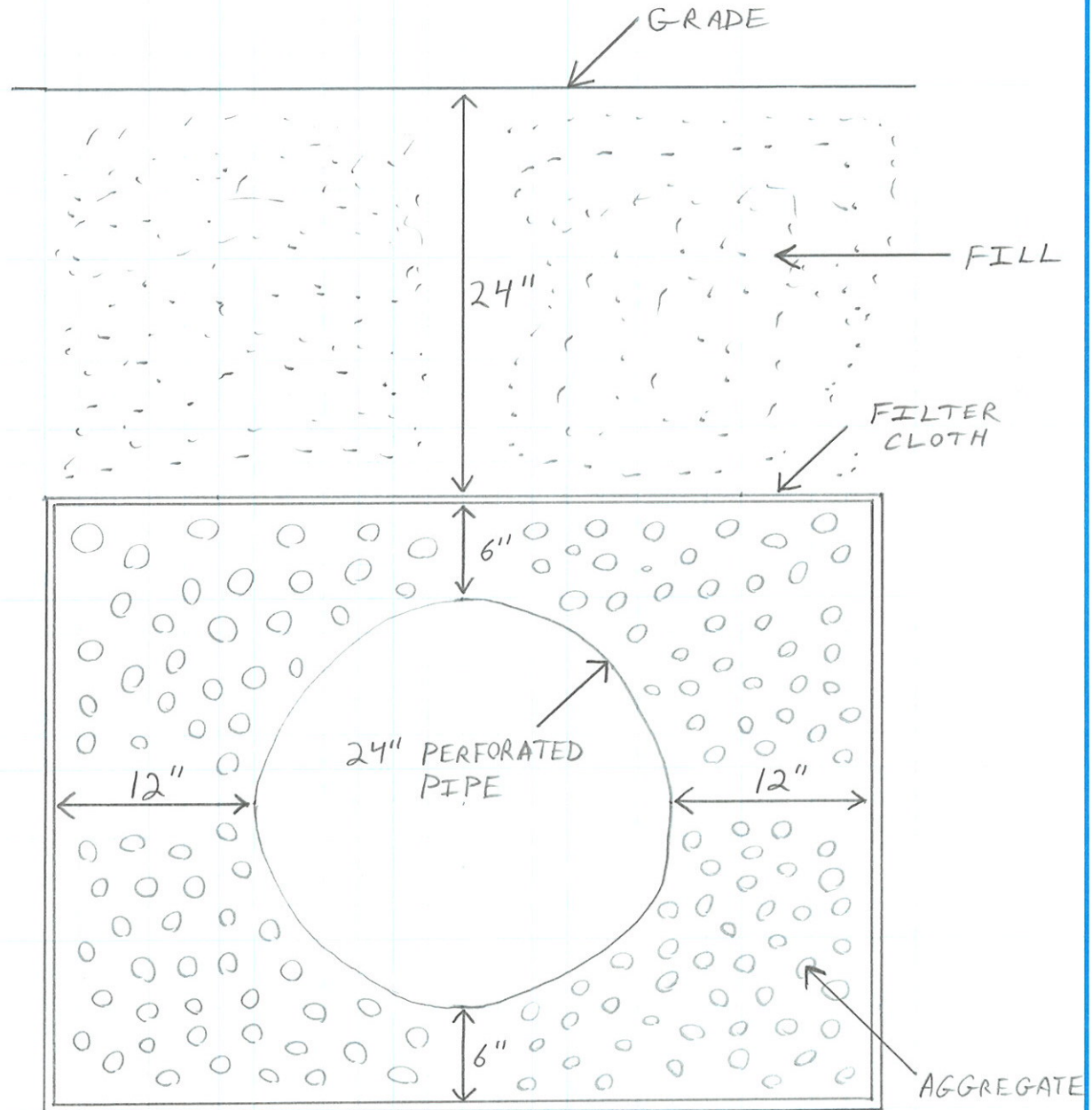
(A) EXFILTRATION TRENCH CROSS SECTION
