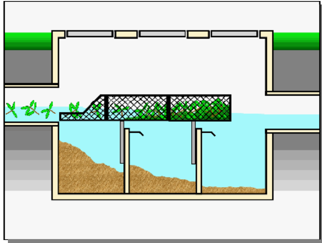
Nutrient Separating Baffle Box (NSBB)
